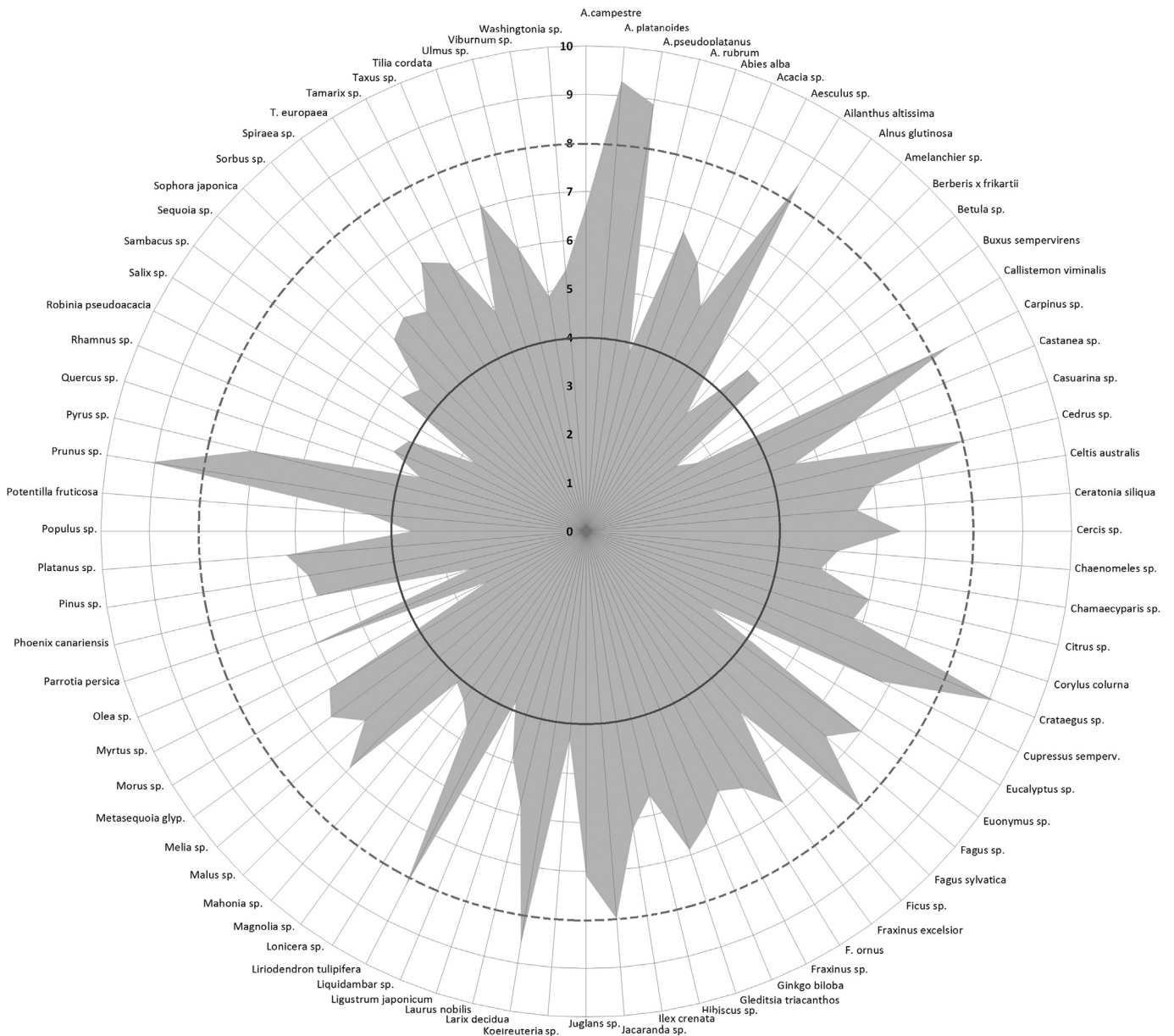
Fig. 2. Species-specific Air Quality Index (S-AQI). S-AQI: 1–4: not recommended (below the tick line); 8–10: recommended plant species for city planting program (over the dotted line).
