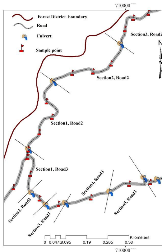
Figure 2. Dividing of road segments to sections based and culvert location in order to road inventory
