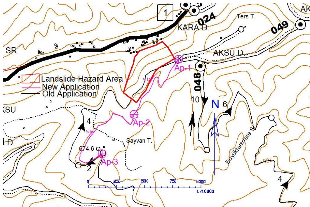
Figure 10. Re-planning the road on the contour map
