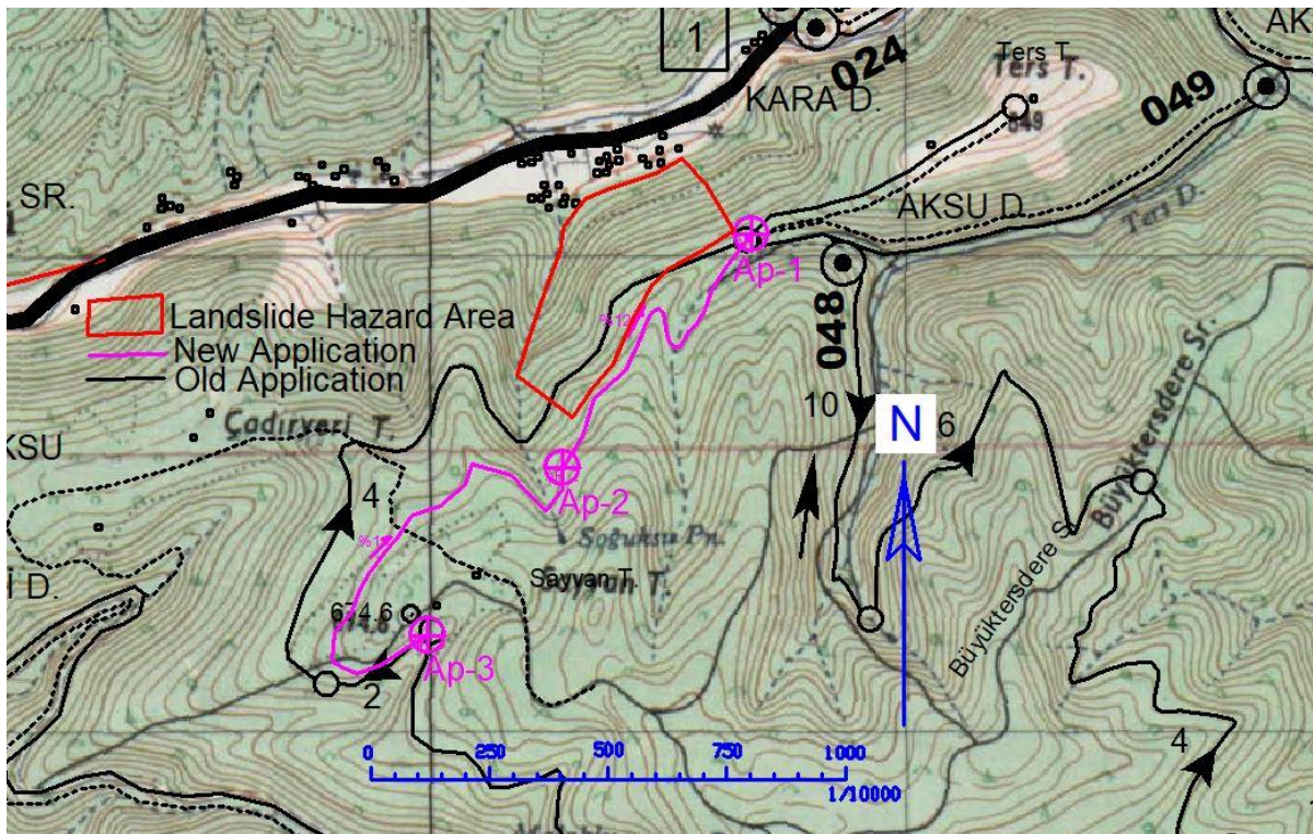
Figure 9. Road section within the landslide hazard area
