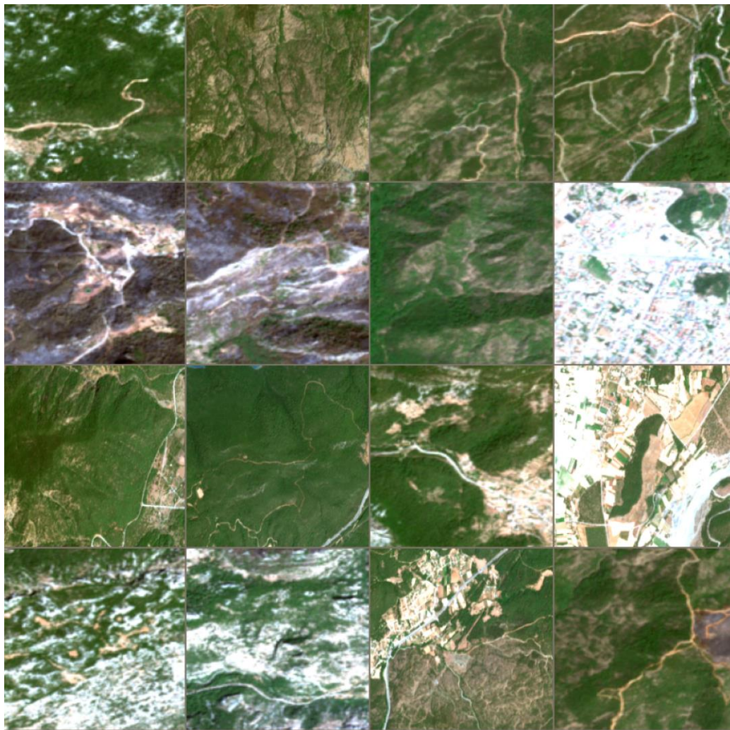
Figure 7. Image matrix
