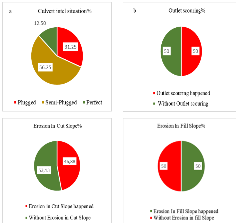
Figure 6. a) Intel situation in pipes, b) Outlet scouring in pipes, c) occurred erosion in culvert's cut slopes, d) the erosion taken place in pipe's fill slopes
