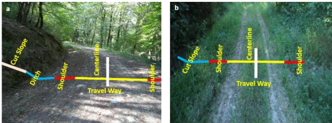
Figure 3. The Road surface elements after 4 years rehabilitation a) the reshaping was conducted in 2017, b) the road surface condition in 2021 without maintenance operation.
