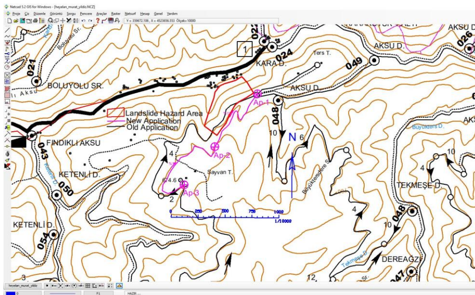
Figure 5. Re-planning the forest road in Netcad 5.2 software
