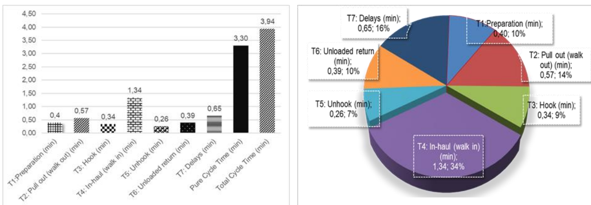
Figure 5. Average values and percentage of work elements in total cycle time.
