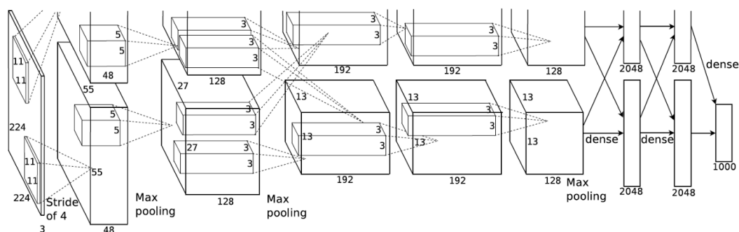
Figure 6. AlexNet architecture
