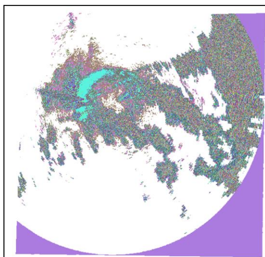
Figure 5. Zonguldak radar image
