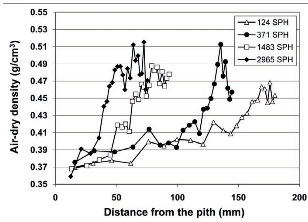
Figure 2: Differences in the radial patterns of variation in wood density at breast height in P. patula trees as affected by age and planting density treatments.
