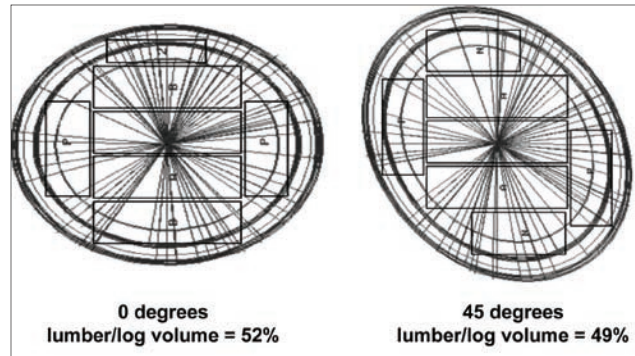
Figure 2— Initial (0-degree) and 45-degree orientations, with conversions, of a log with an ellipticity ratio of 0.80.
