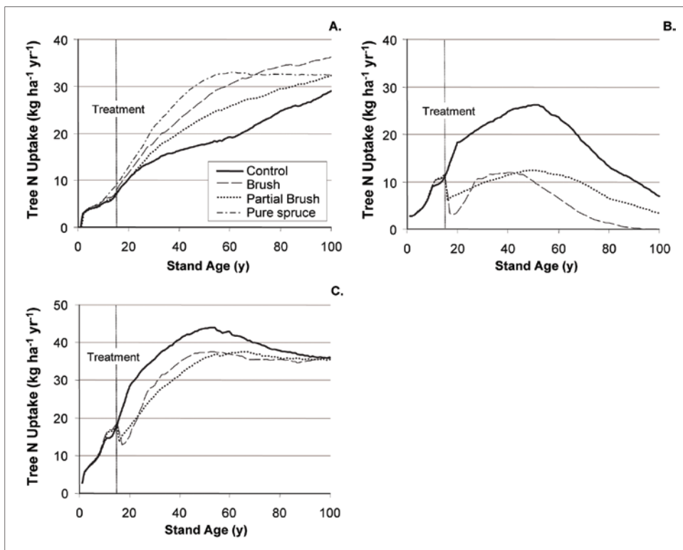
Figure 3. Simulated annual nitrogen (N) uptake for A) spruce and B) aspen and C) total tree for the two aspen brushing treatments and the control in the spruce-aspen mixedwood stand type.
