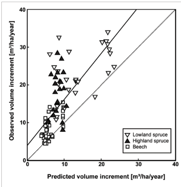
Figure 2. Predicted vs. observed volume increments following thinning using the current model setup.
