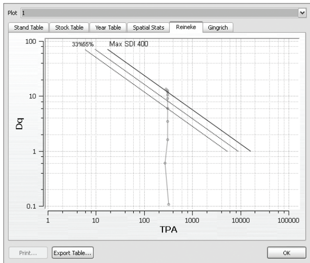
Figure 14— An example of the Sylview Program (Scott 2006). The stand illustrated is cherrybark oak ( Quercus pagoda Raf. )-sweetgum ( Liquidambar styraciflua L. ) from Mississippi, USA. This is a standard density-management diagram of the model’s data from this plot.
