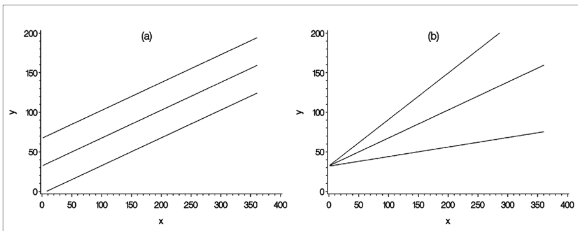
Figure 6. Difference equation growth curves generated from eqs. [11] (left) and [12] (right), based on the estimated coefficients ( b_0 = 31.9217 , b_1 = 0.35189 ) for the cumulative function y = b_0 + b_1x , and given y_1 values of 50, 85 and 120 at a fixed reference x_1 value of 150.
