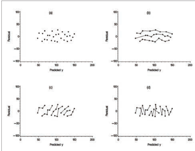
Figure 5. Residual plot (a) and residual trajectories (b, c, d) from the ordinary least squares fits of the simple linear regression y = b_0 + b_1x on the data shown in Figure 2.
