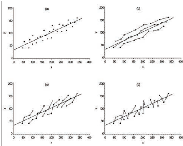
Figure 2. Twenty-eight hypothetical data points unconnected (a), and connected in different ways (b, c and d). The data points and the connected trajectories in (b), (c) and (d) are listed in Table 1. The simple linear regression line ( y = 31.9217 + 0.35189x ) obtained from the ordinary least squares fit is overlaid on the data. Note that the same data points appear in all four graphs.
