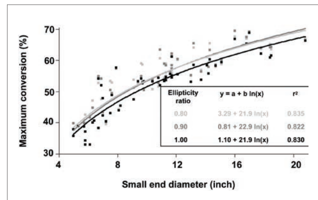
Figure 4— Logarithmic regressions demonstrating the relationship between maximum conversion and log small-end diameter by ellipticity ratio.
