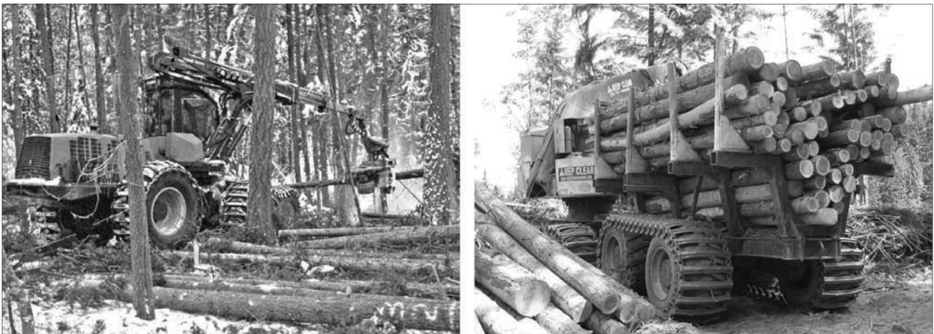
Figure 3. Left image: Harvesting machine processing a tree into logs in a thinning operation. Right image: Forwarder at the landing with a load of logs.
