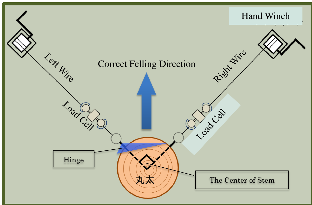
Fig. 3 Conceptual Diagram of Pulling Test
