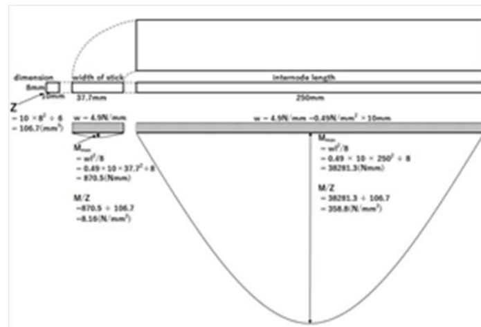
Figure 3: Consideration of maximum bending moment
