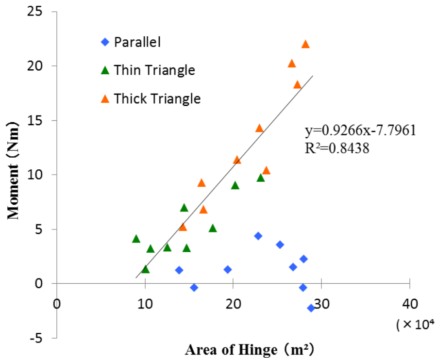
Fig.8 Relation between moment and area of hinge
