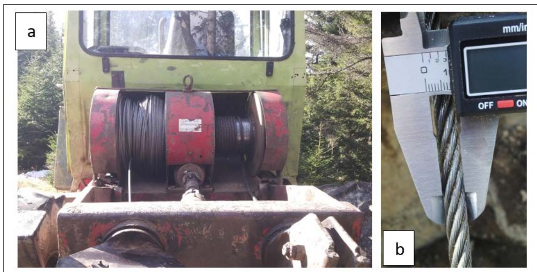
Figure 1. Mini yarding components. Forest tractor (a), main cable (b)
