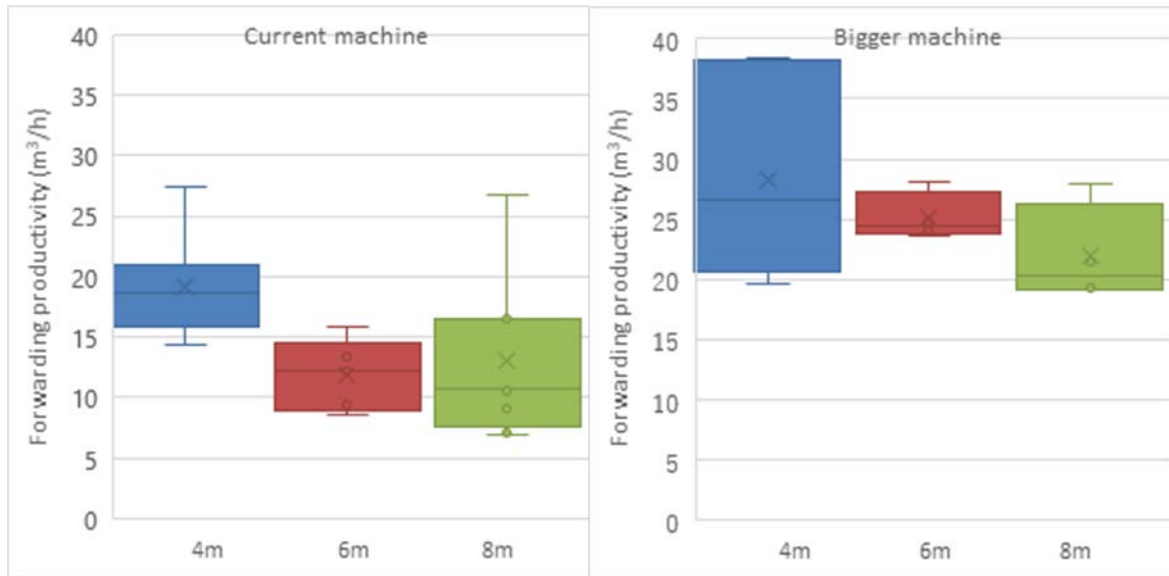
Figure 7. Forwarding productivity for each log length class
