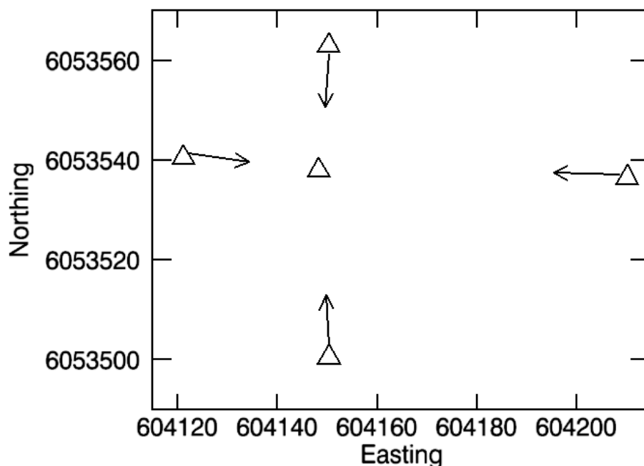
Figure 1: ILRIS scan configuration with 4 scan locations looking into centre of the EVI scan location from north, east, south and west ILRIS scan locations. Each ILRIS scan location has two scans: one parallel with ground and another inclined vertically and aimed into the canopy.
