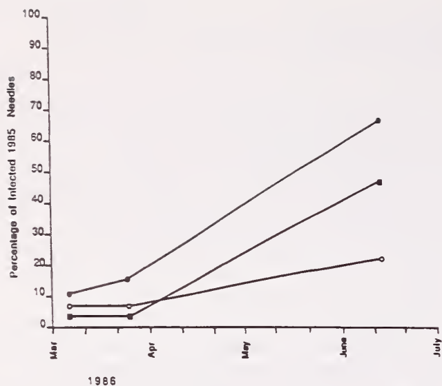
Treatments: ●-Check ○-2.3 kg a.i./ha 6 June, 20 Aug., 9 Oct. 1985 + 24 March 1986. ■-9.3 kg a.i./ha 6 June 1985 + 4.7 kg a.i./ha 24 March 1986. Sampling dates: 5 March, 24 March, 12 June 1986.
