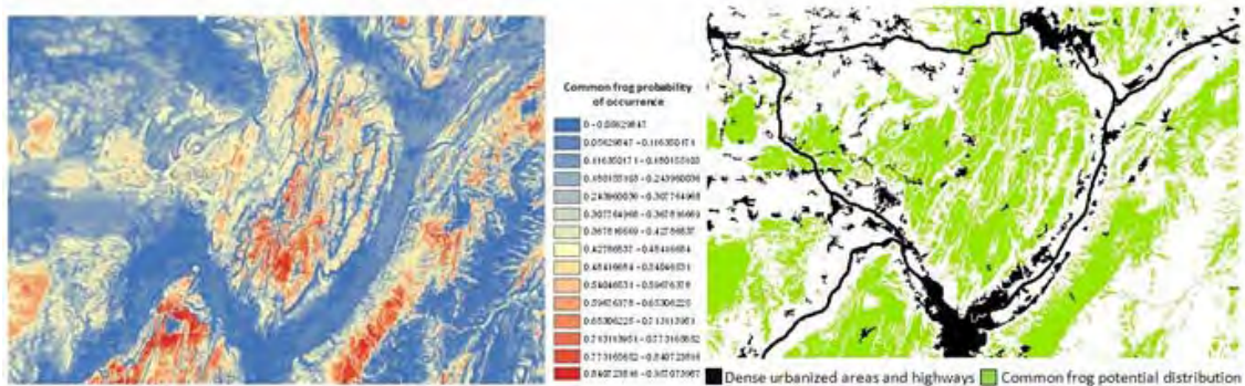
Figure 2: Probability of occurrence distribution for the common frog with the maximum entropy modelling and resulting potential distribution of the common frog (10 percentile training presence of 0.339 as the probability threshold) (area of 4067 km 2 ).
