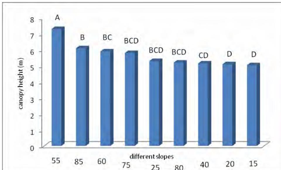
Figure 8: canopy height in different slopes
