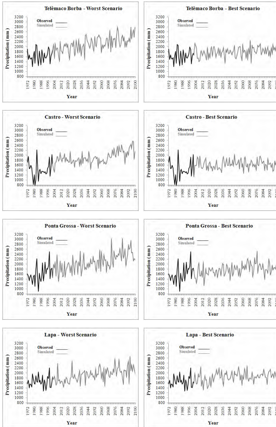
Figure 3 - Precipitation scenarios simulated by PGCLIMA_R for the year 2100, considering the best and worst outlook projected by the IPCC.
