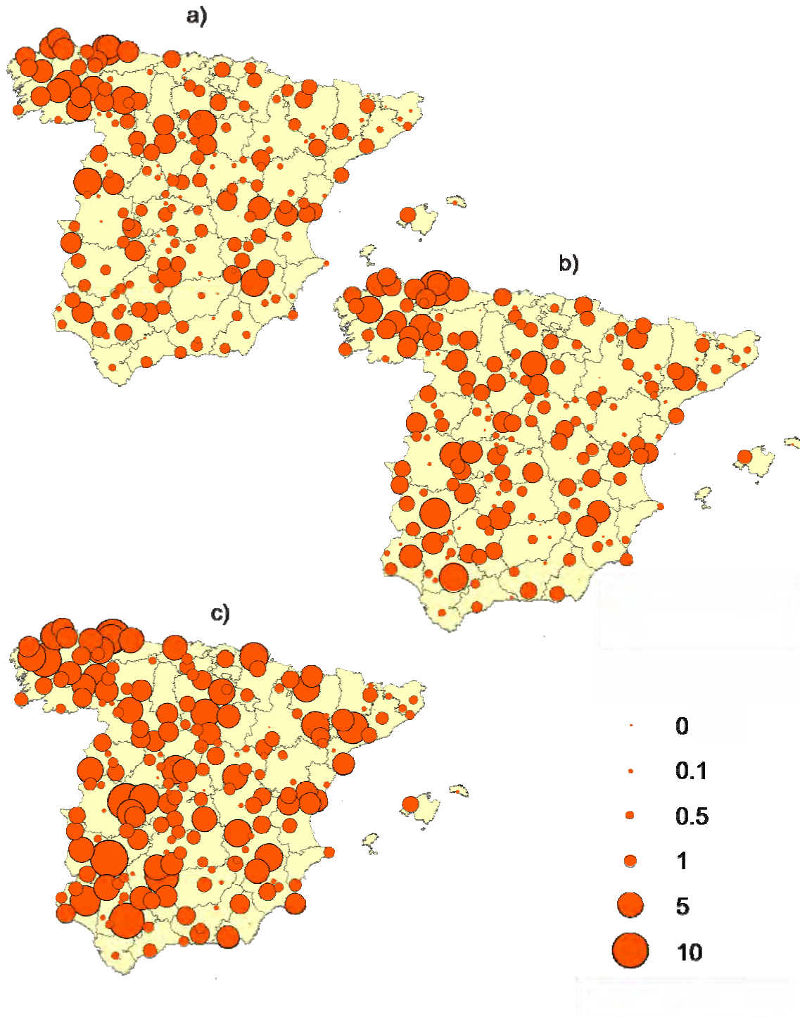
Figure 1: Monitoring of Forest Landscape Vulnerability (FLV) in 206 squares of SISPARES approach along three dates: (a) 1956, (b) 1984 and (c) 1998. The point size indicates the value of FLV.
