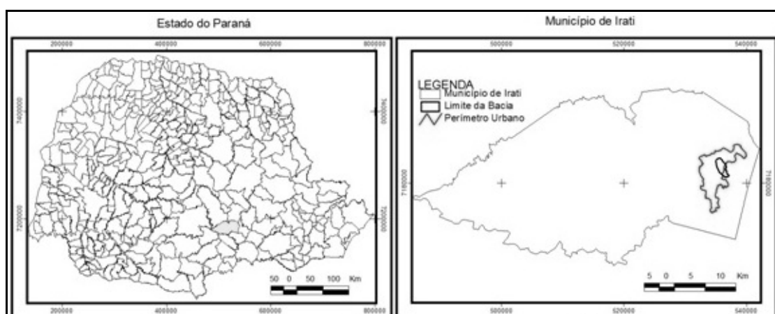
Figure 1 - Location of the Hydrographical Basin of Arroio dos Pereiras Org: Campos, 2006.
