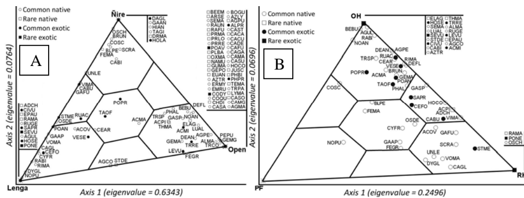
Figure 2: DCA for the analysis of plant species distribution: (A) among Nothofagus pumilio forests (Lenga), N. antarctica forests (Ñire) and grasslands and peat-lands (Open); (B) among primary unmanaged N. pumilio forests (PF), recently harvested forests (1-5 years) (RH) and old harvesting (>5 years) (OH). Codes for plant species appeared in Table 1.
