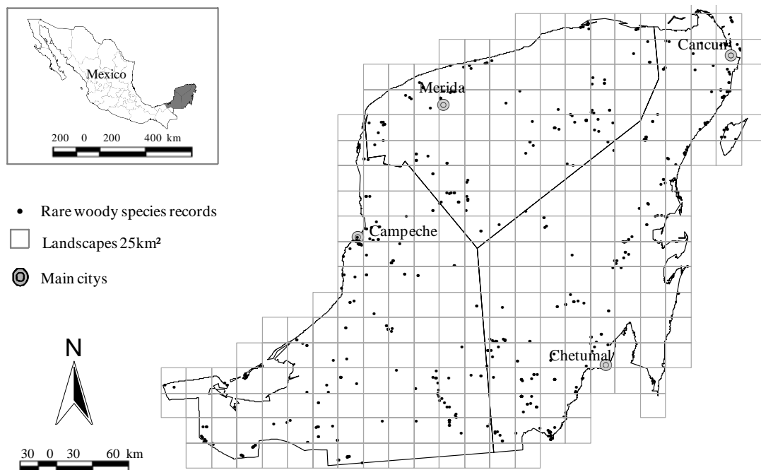
Figure 1: Study area and rare woody species records within 25 \text{ km}^2 landscapes.
