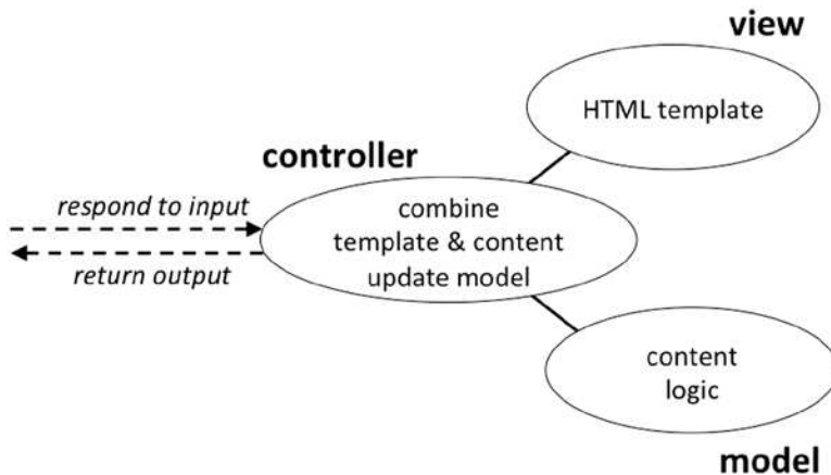
Figure 7-2. Model-view-controller
